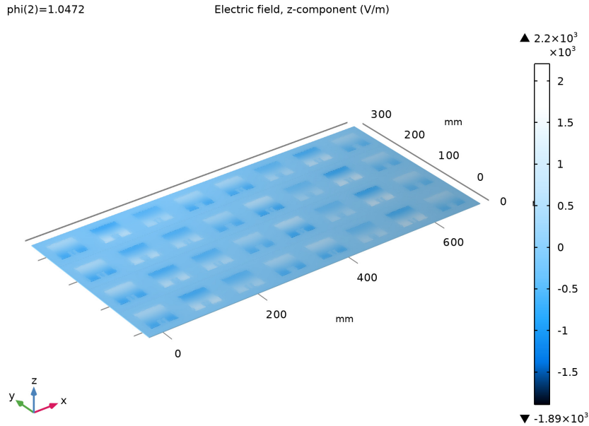
Figure 4: E_z plot showing the color variation at each array column.
