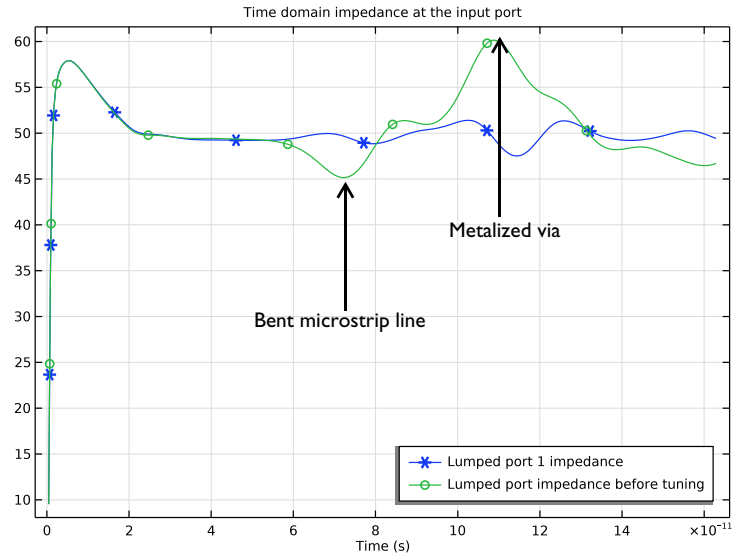
Figure 3: The time-domain impedance at lumped port 1. After tuning, the measured impedance is closer to 50 \Omega .
