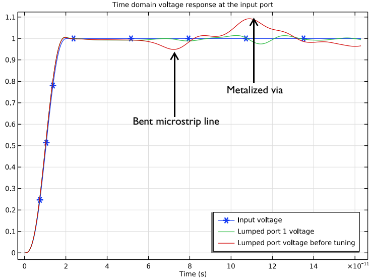
Figure 2: The time-domain voltage measured at lumped port 1. The undesired voltage fluctuation from the discontinuities is suppressed after tuning.
