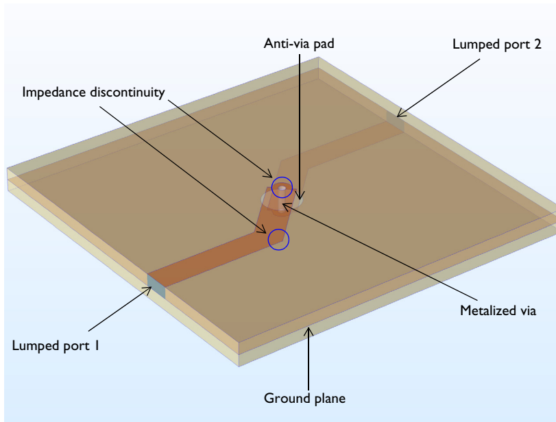
Figure 1: A microstrip line on a multilayer circuit board. A 20 mil (0.508 mm) microwave substrate is used for each dielectric layer. The ground plane with an anti-via pad is located between two dielectric layers. The top and bottom microstrip lines are connected with a metalized via hole.
