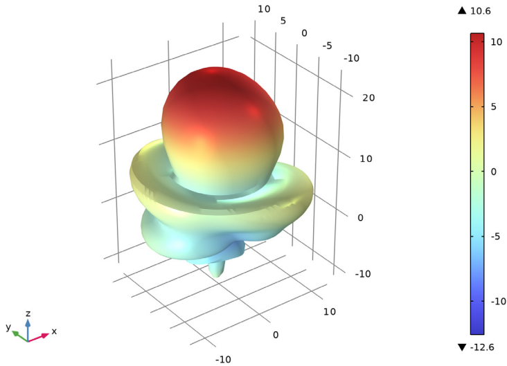
Figure 5: The 3D far-field pattern looks like that of an end-fire array along the z-axis backed by a ground plane.
