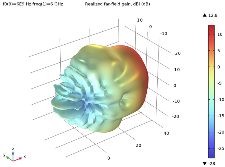
Figure 3: 3D far-field radiation pattern that is directive toward the open aperture.
