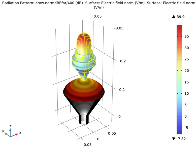
Figure 2: 3D far-field radiation pattern in dB, visualized with the grid above the lens. The E-field norm is focused gradually toward the center.
