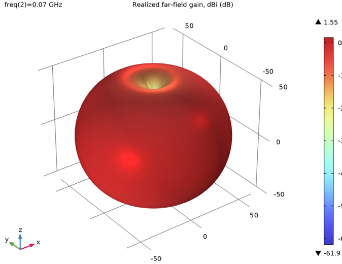
Figure 4: 3D far-field pattern at 70 MHz. The pattern resembles that of a typical half-wave dipole antenna.
