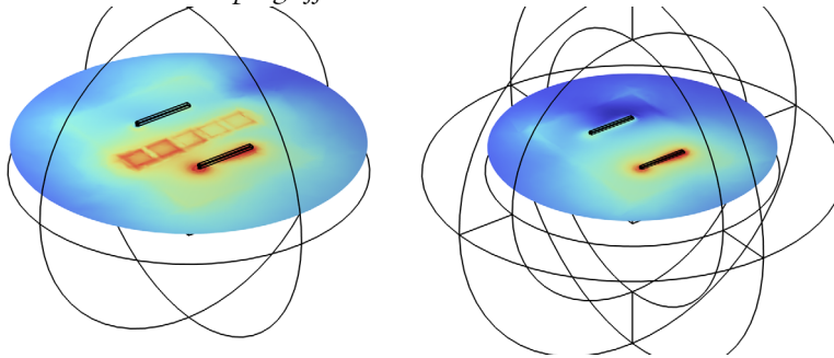
Figure 3: Electric field with EBG (left) and without EBG structures (right).
