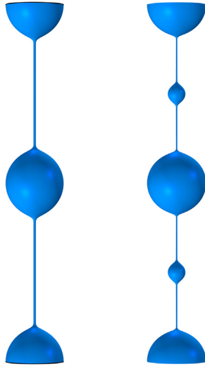
Figure 3: Filament shapes for \beta = 0.25 , Oh = 3.16 , De = 94.9 , and t/\tau = 300 (left) and \beta = 0.25 , Oh = 0.4 , De = 0.8 , and t/\tau = 19.75 (right).
