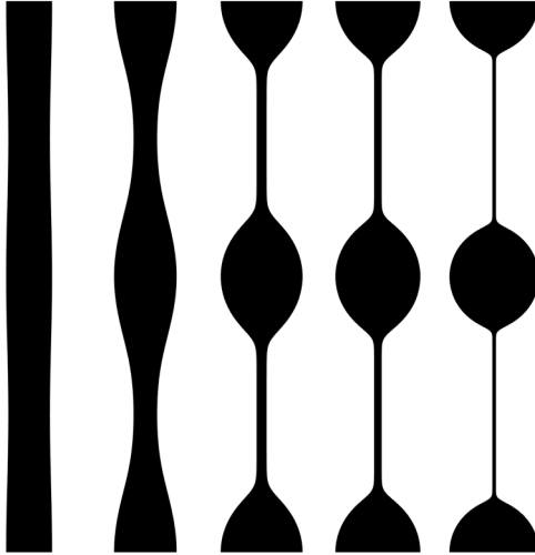
Figure 1: Filament profiles at 5 different dimensionless times: 0, 20, 30, 100, and 300.
