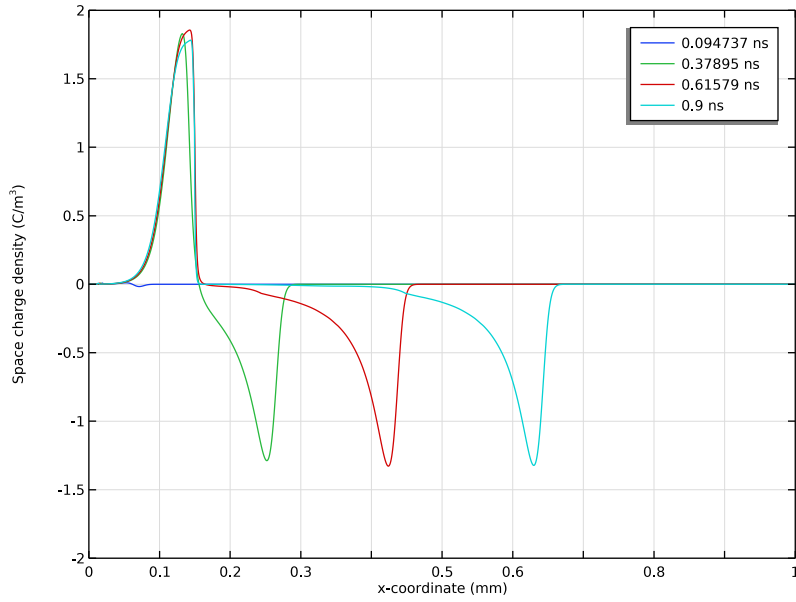
Figure 3: Space charge density for four time instants during the streamer propagation.
