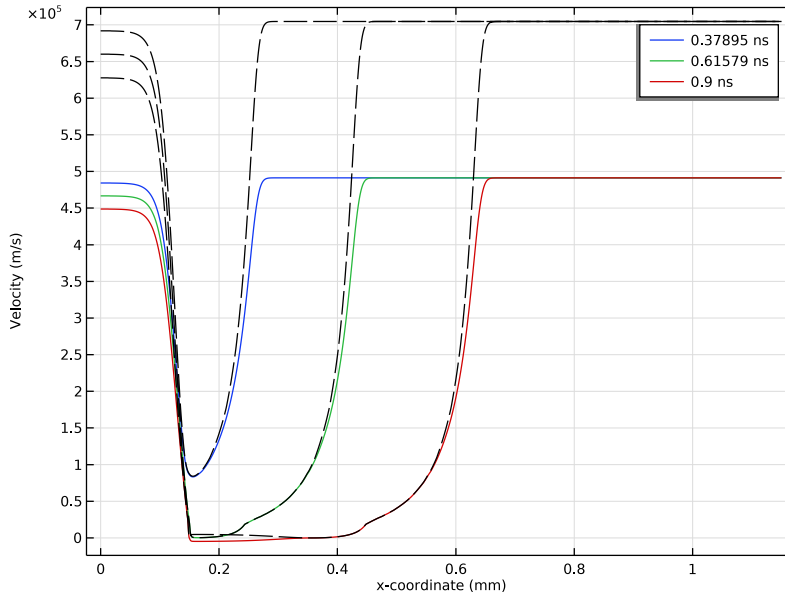
Figure 5: Electron drift velocity (colored solid lines) and velocity computed using Equation 4 (black dashed lines) for three time instants during the streamer propagation.
