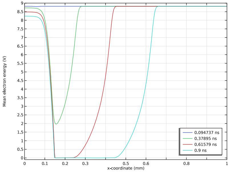
Figure 4: Mean electron energy for four time instants during the streamer propagation.
