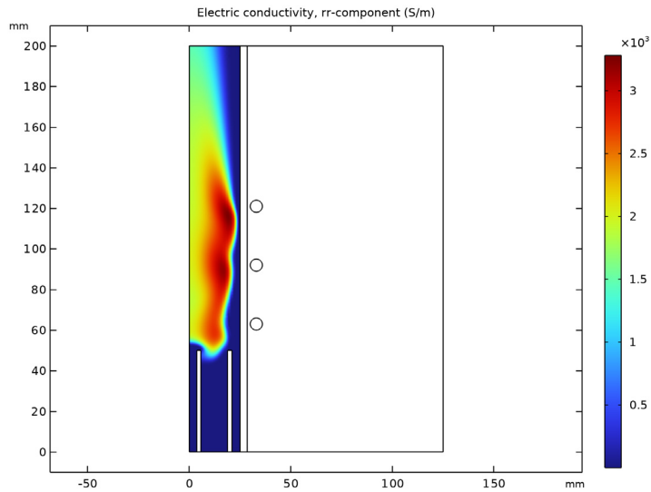
Figure 5: Plot of the plasma electric conductivity.
