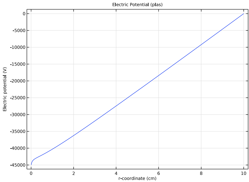
Figure 5: Spatial profile of the electric potential.
