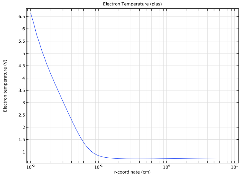
Figure 4: Spatial profile of the electron temperature.
