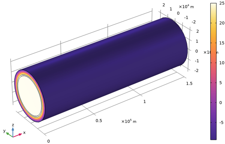
Figure 4: Temperature distribution.
