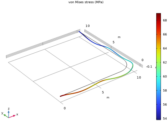
Figure 3: von Mises stress distribution along the deformed pipe. The deformation is magnified.
