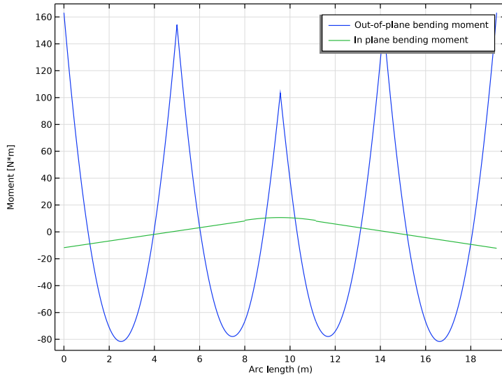
Figure 5: Bending moments.
