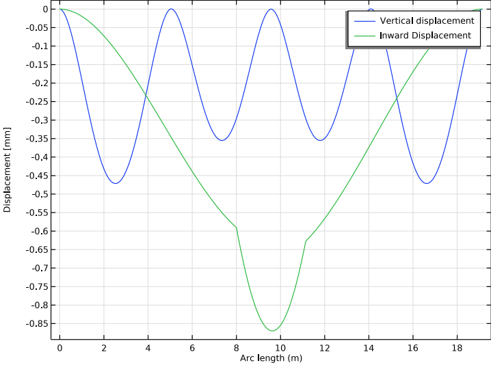
Figure 4: Pipe displacement.
