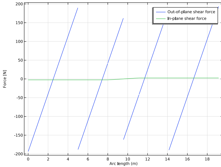
Figure 6: Shear forces.
