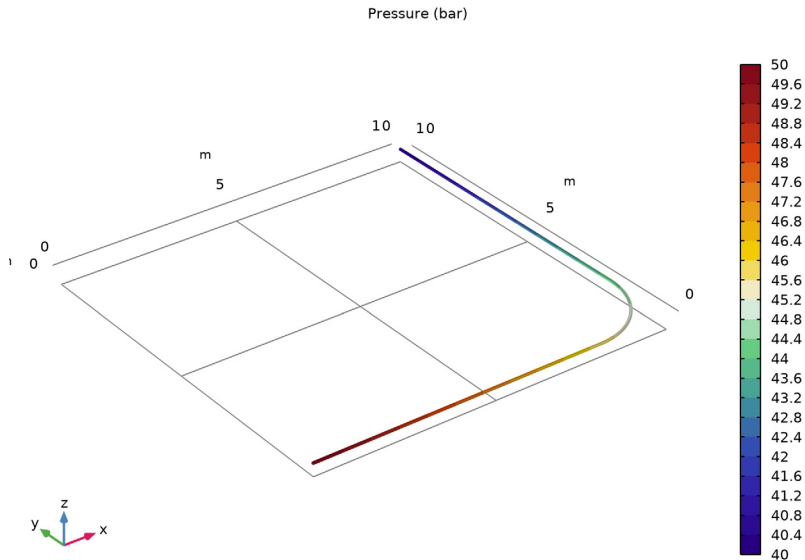
Figure 2: Pressure distribution.
