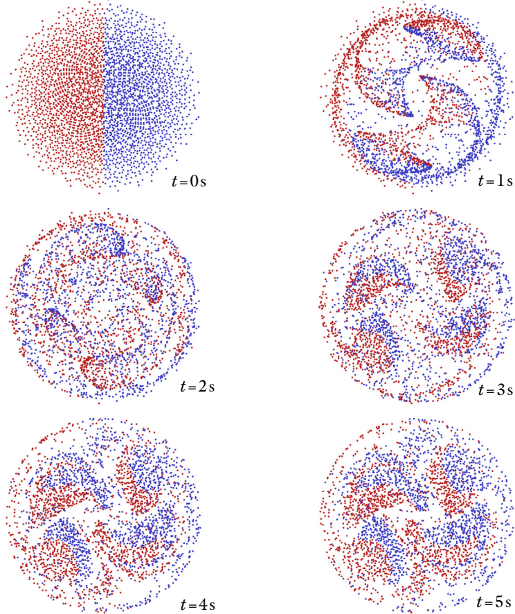
Figure 5: Plot of the particle position in the xz -plane at different times. The red particles had an initial position of x < 0 and the blue particles had an initial position of x > 0 .
