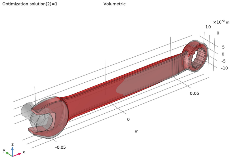
Figure 3: The shape of the wrench is optimized by removing material from the head and the handle. Furthermore, the middle part is thicker in the z direction and the kink near the handle has been straightened out.
