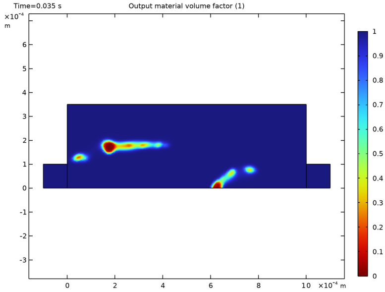
Figure 2: The filtered material volume factor is plotted for the optimized design.
