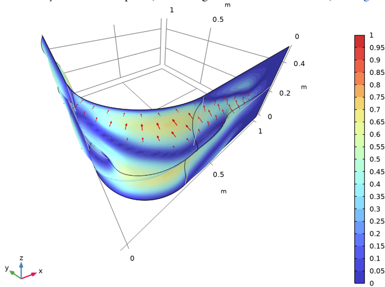
Figure 2: The default shape optimization plot shows the edges of the old geometry in gray together with a surface plot of the relative normal boundary displacement in colors. The actual displacement is shown with red arrows.
