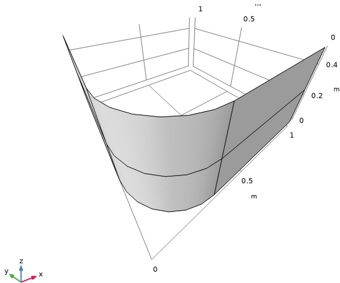
Figure 1: The initial geometry is shown. The displacement and rotation is fixed at the leftmost edge of the shell. The shape deformation of this edge is restricted to the xz -plane.
