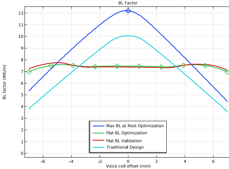
Figure 4: BL Curve comparison. The plot includes the BL curve of the Optimization maximizing the BL factor at the resting position (blue), the optimization creating a flatter BL curve (green), the validation model using the results from the second optimization (red), and the results of a traditional design with similar dimensions and a larger iron volume (light blue).
