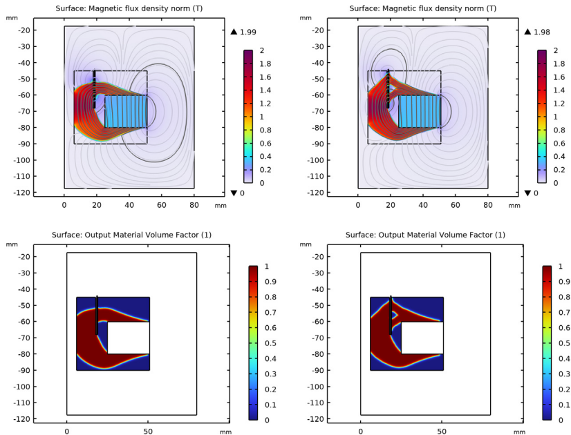
Figure 2: Magnetic flux density norm (top) and Output material volume factor (bottom) for the studies maximizing the BL factor at the resting position (left) and creating a flatter BL curve (right).
