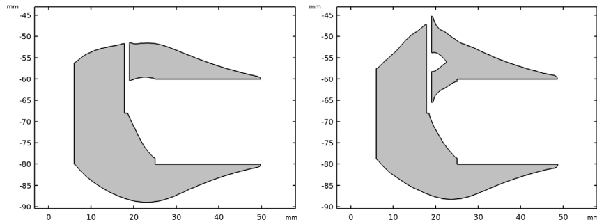
Figure 3: Filtered results for the studies maximizing the BL factor at the resting position (left) and creating a flatter BL curve (right).
