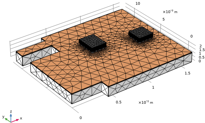
Figure 6: Meshed geometry.
