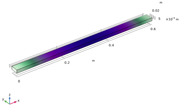
Figure 3: Eigenfrequency and normalized eigenfunction for a prestressed rail.
