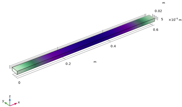
Figure 2: Eigenfrequency and normalized eigenfunction for a stress-free rail.
