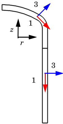
Figure 2: Orientation of the local material coordinate system. The second principal direction is oriented in the circumferential direction, perpendicular to the rz -plane.
