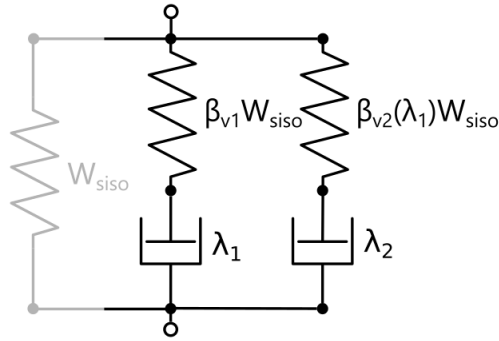
Figure 2: Rheology of the Bergstrom–Bischoff material model.
