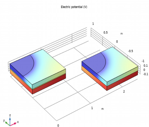
Figure 2: Potential distribution in the modeled device. The value of the potential loss over the device at a current of 0.3\text{ A} is almost identical in the two models: the full model (left) and thin-film approximation (right).
