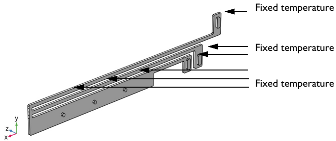
Figure 3: Heat-transfer boundary conditions.
