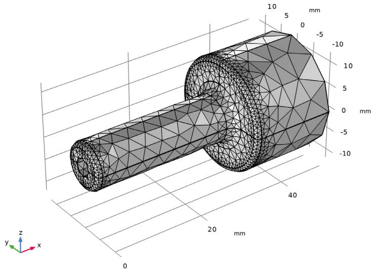
Figure 1: The geometry and mesh of the full model.
