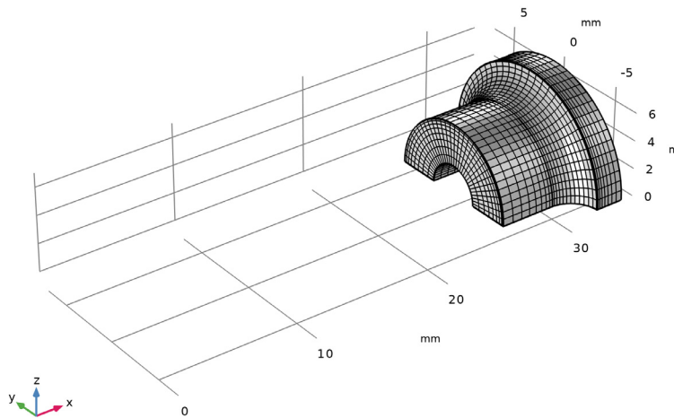
Figure 2: The geometry and mesh of the submodel.
