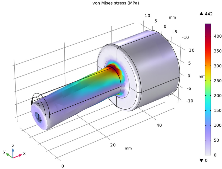
Figure 3: Stress distribution in the full model.
