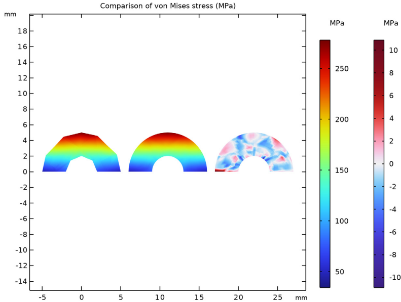
Figure 7: Stress distribution over one of the cuts. Full model (left), submodel (center), and their difference (right) are shown. Note the separate color bar for the difference.
