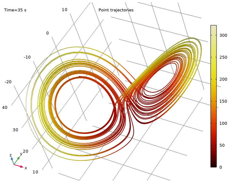
Figure 2: The typical pattern for a Lorenz attractor visualized using a Point Trajectories plot of the phase space.
