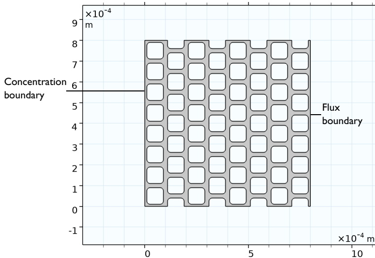
Figure 1: Artificial porous structure.
