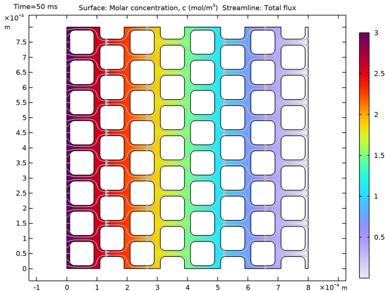
Figure 2: Concentration profile and flux streamlines in the modeled artificial porous structure at t = 0.05 s.
