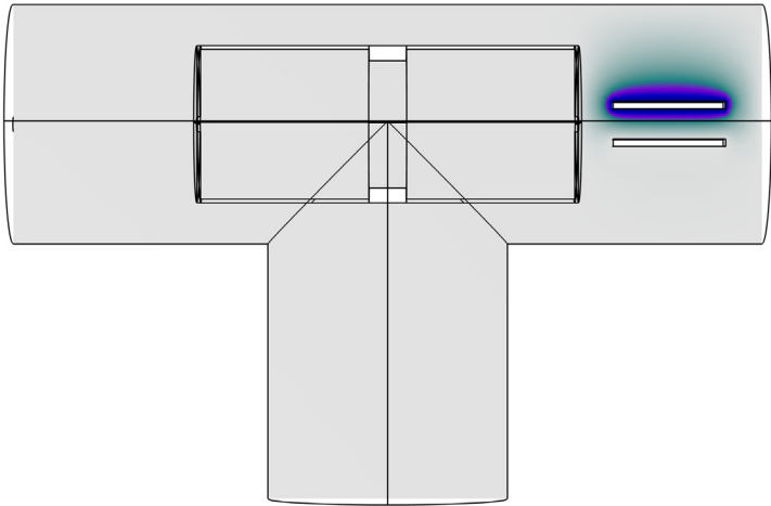
Figure 3: Electric potential in the vacuum housing.
