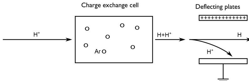
Figure 1: Schematic of a simplified charge exchange cell neutralization process.
