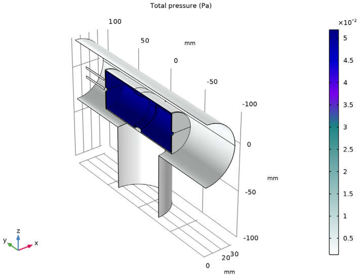
Figure 4: Pressure in the apparatus.
