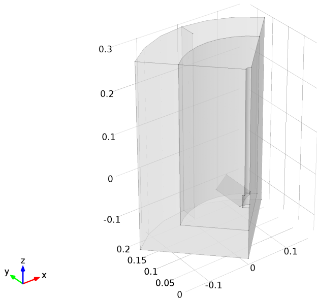
Figure 2: Geometry used in the simulation.
