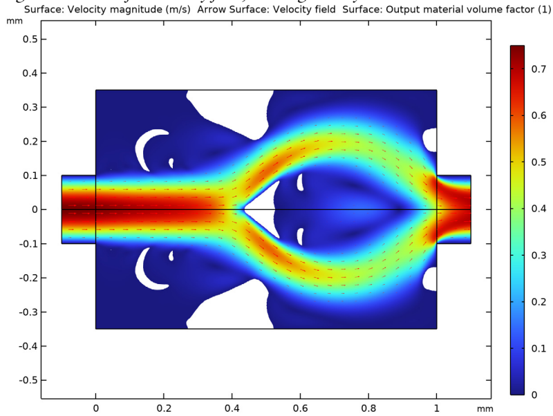
Figure 4: Forward flow, optimized topology.
