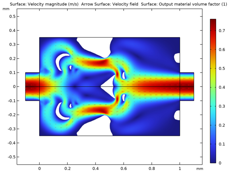
Figure 5: Reverse flow, optimized topology.
