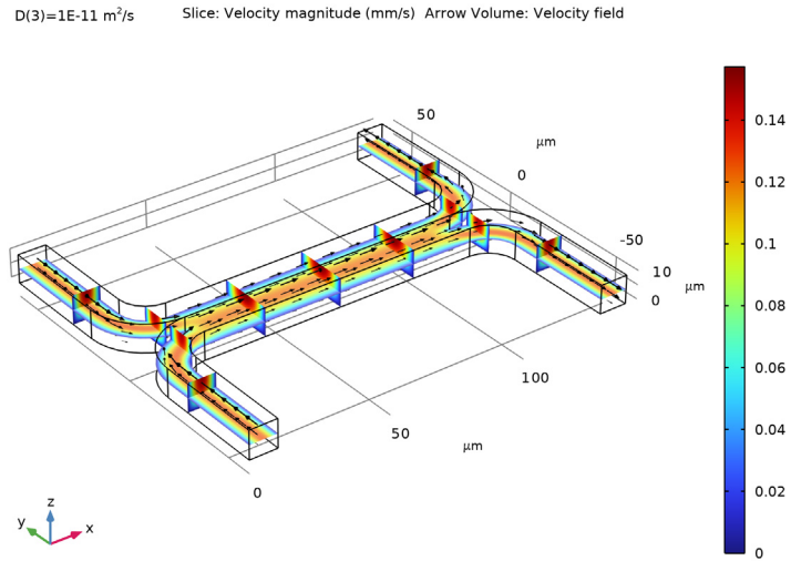
Figure 3: Flow velocity field.
