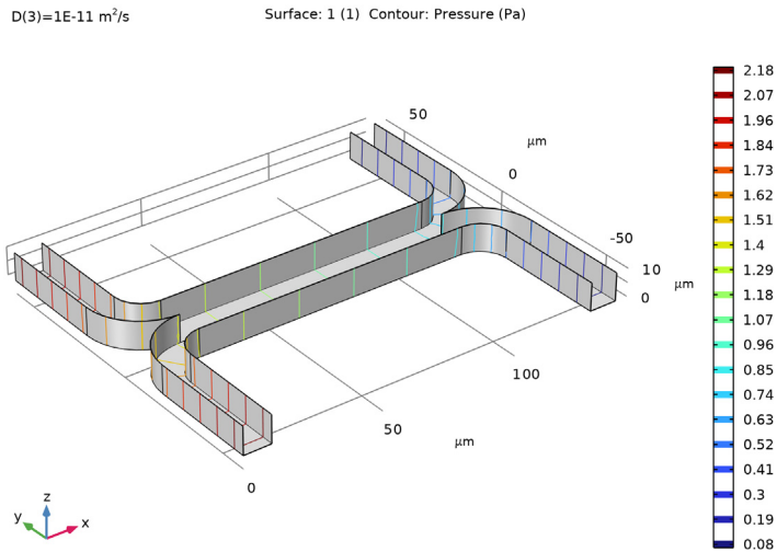
Figure 4: Pressure distribution on the channel walls.
