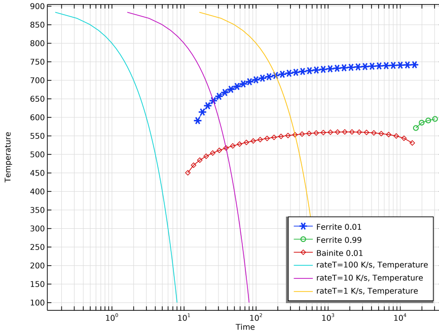
Figure 3: Computed CCT diagram showing the curves for 1% formed fraction of ferrite and bainite.
