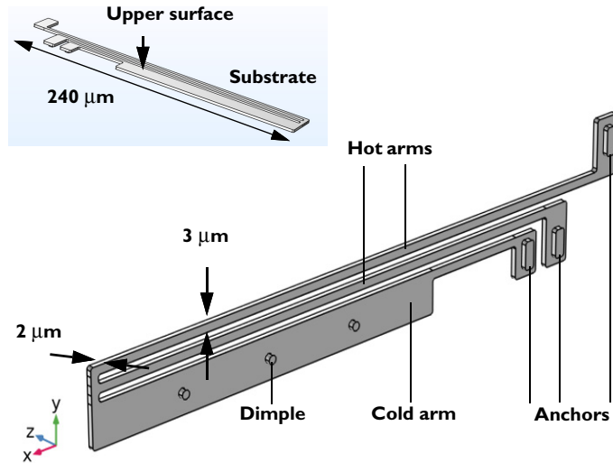
Figure 1: The thermal microactuator.
