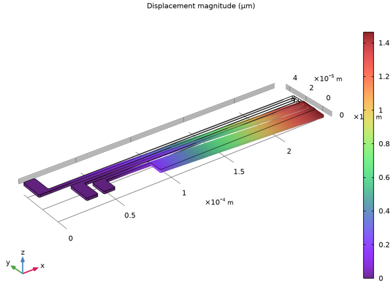
Figure 6: Displacement in the thermal actuator (here exaggerated by a factor of about 6.6).
