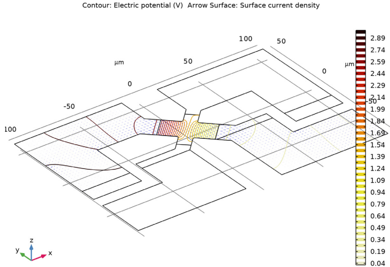
Figure 5: Arrows: Current density, Contours: Electric Potential, for a device driven by a 3 V bias with an applied pressure of 100 kPa.
