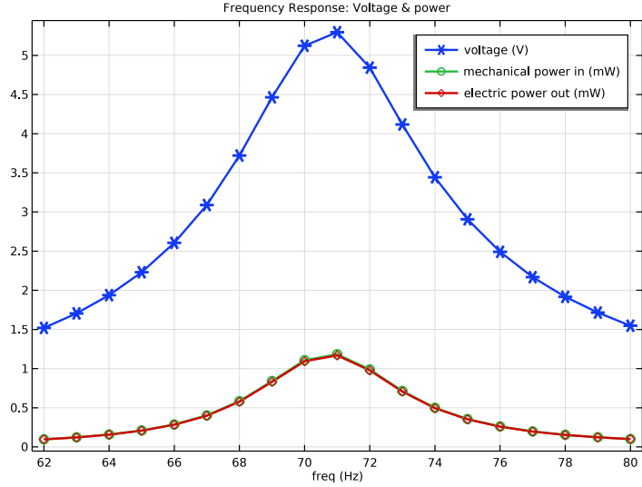
Figure 2: Energy harvester input mechanical power and the power harvested (in mW) as well as the peak voltage induced across the piezoelectric bimorph (in V) vs. excitation frequency. The load impedance is 12 kΩ and the acceleration magnitude is 1 g.
