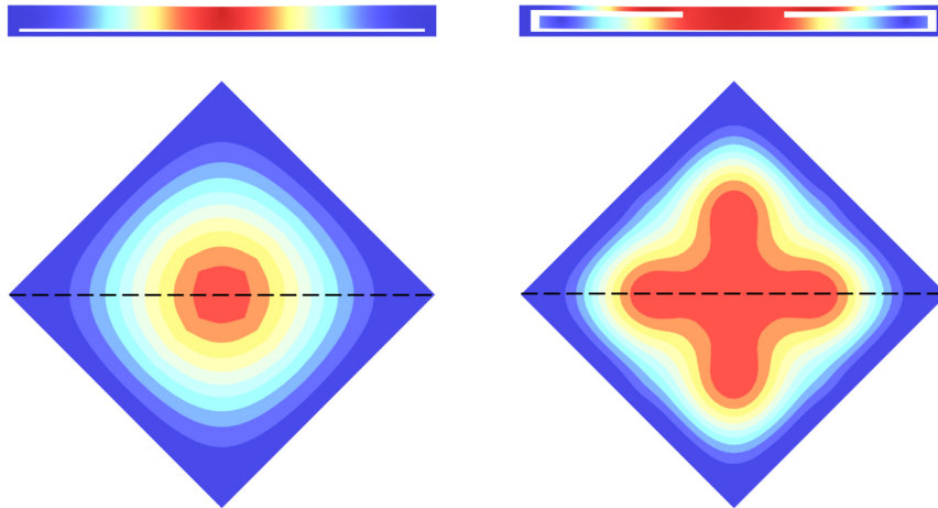
Figure 7: CMUT cross sections along the diagonals (dashed line) for the standard design (Top-Left) and the piston-shaped design (Top-Right). Displacement across CMUT for the standard design (Bottom-Left) and the piston-shaped design (Bottom-Right). The piston-shaped suspended mass increases displacement uniformity.
