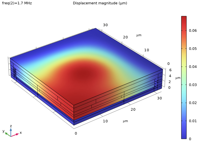
Figure 5: The solid displacement of the structure with a harmonic perturbation at 1.7 MHz. Maximum displacement is at the center of the device and is about 65 nm.
