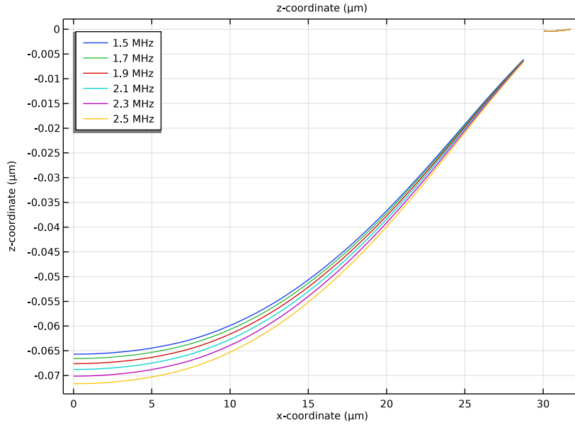
Figure 4: Profile of the top electrode as a function of frequency. Maximum displacement is at the center of the device and is about 65 nm at 1.7 MHz.
