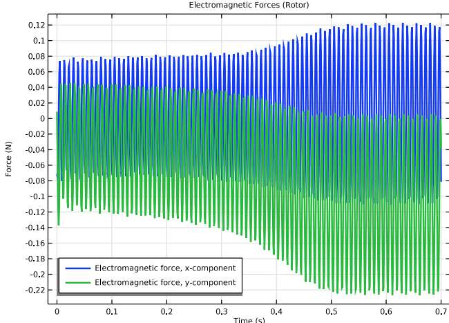
Figure 7: Electromagnetic forces in the rotor in transverse and axial directions.
