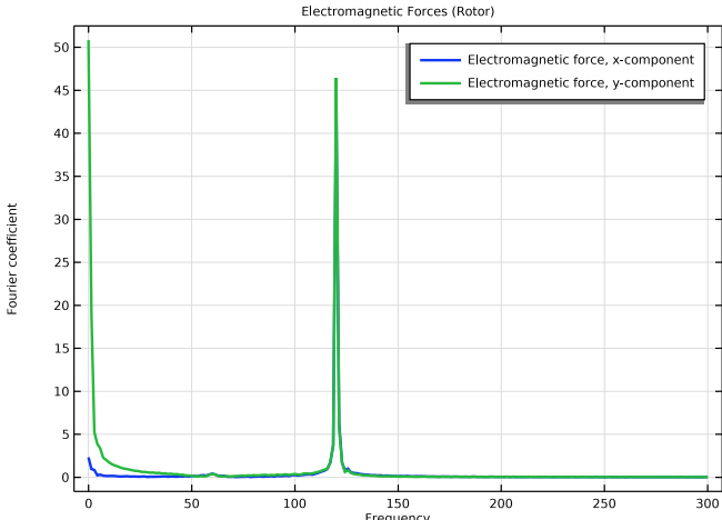
Figure 8: Frequency spectrum of electromagnetic forces in the rotor.
