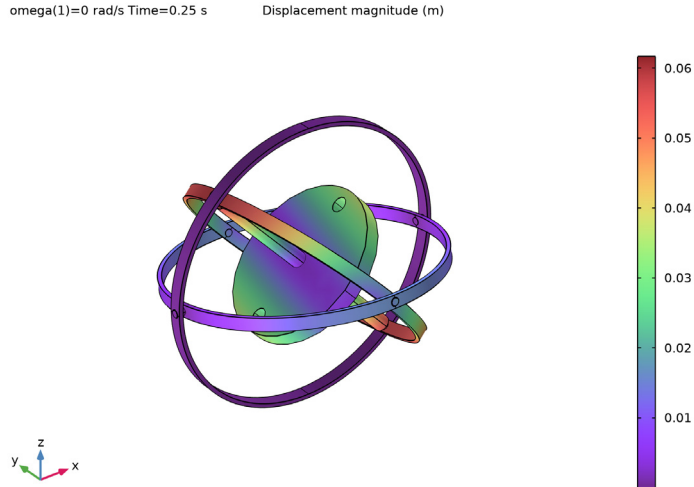
Figure 2: Displacement of the gyroscope components at t = 0.25 sec when the disc is not spinning.
