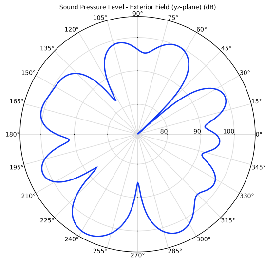
Figure 10: Far-field sound pressure level at a distance of 1 m in the yz-plane at 2000 Hz.
