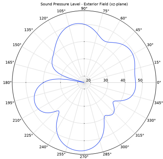
Figure 7: Exterior-field sound pressure level in the xz -plane at a distance of 2 m.
