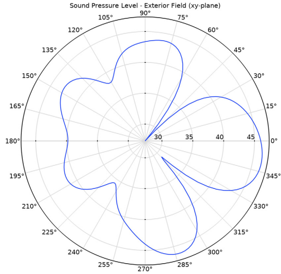
Figure 6: Exterior-field sound pressure level in the xy -plane at a distance of 2 m.
