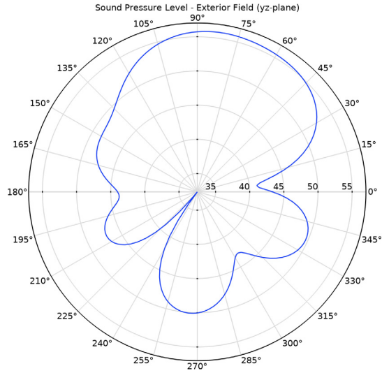
Figure 8: Exterior-field sound pressure level in the yz -plane at a distance of 2 m.
