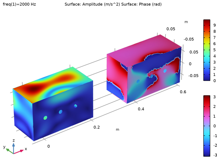
Figure 3: Amplitude and phase of normal acceleration of housing .
