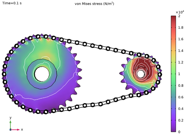
Figure 8: The von Mises stress distribution in the chain drive, at t = 0.1 s
