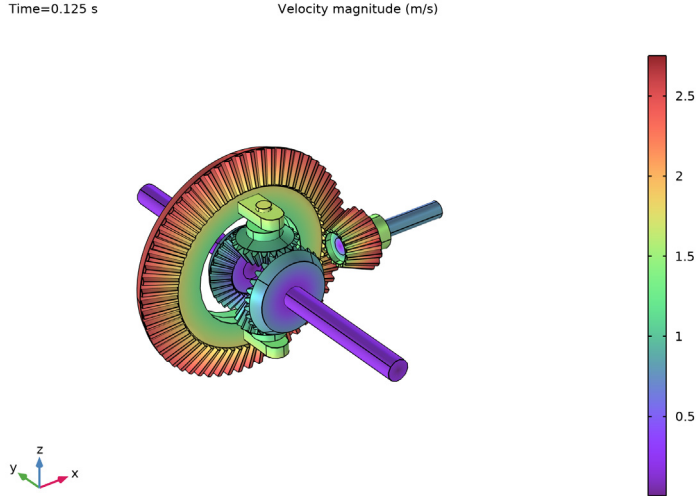
Figure 2: Speed of the different components in a differential after 0.125 s.
