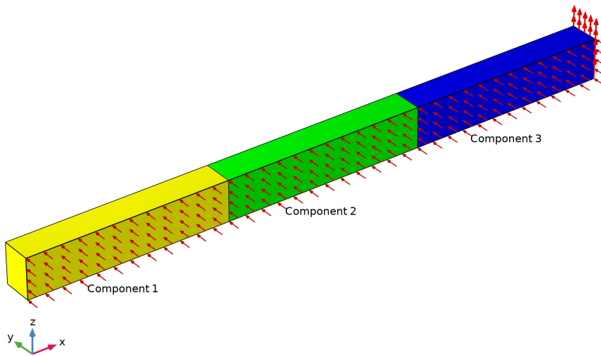
Figure 1: Geometry of the model showing three components and the applied loads.
