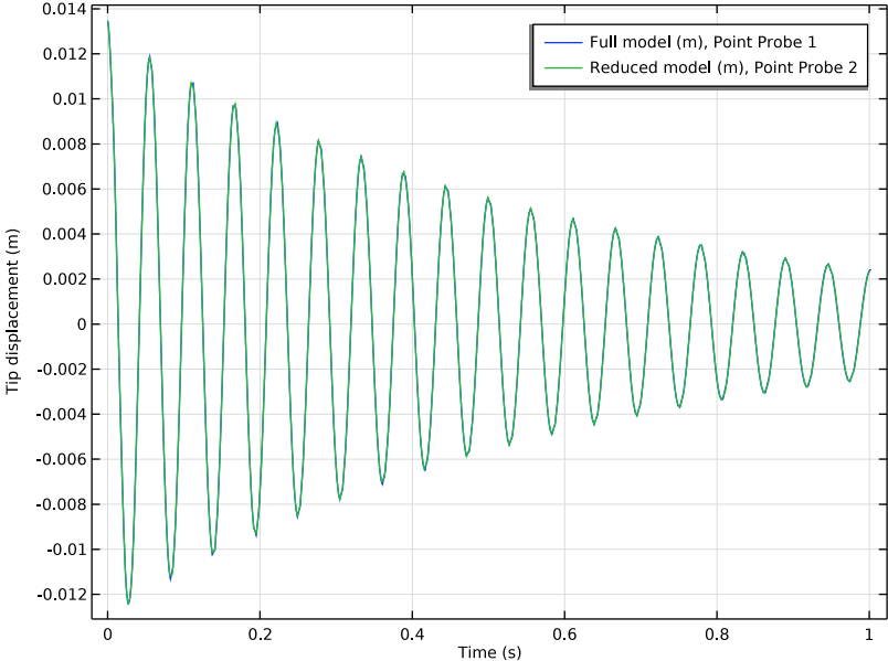
Figure 4: Tip displacement for both configurations of the analysis.
