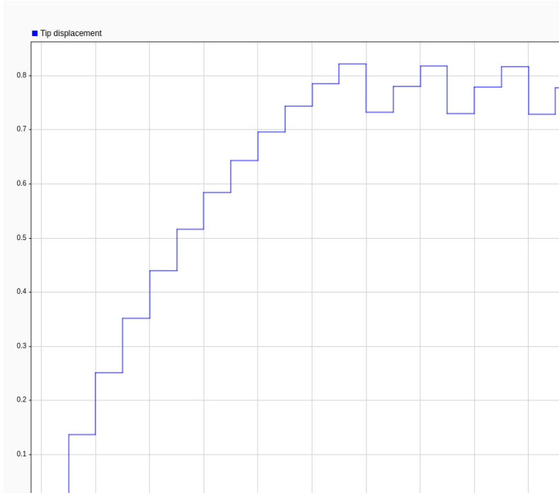
Figure 2: Actuator tip displacement at communication time.
