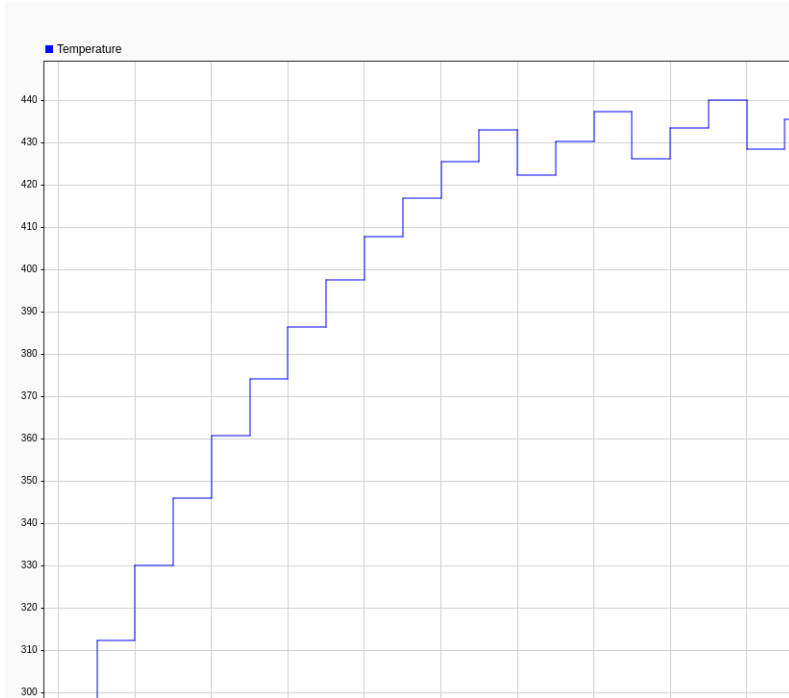
Figure 5: Actuator maximum temperature versus time.
