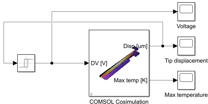
Figure 1: Simulink diagram of the thermal actuator controller.
