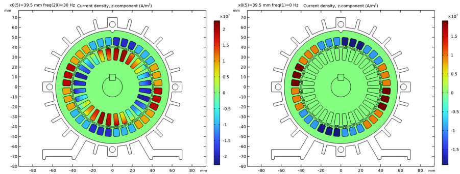
Figure 7: Current density, z-component, at 0% (left) and 5% slip (right).
