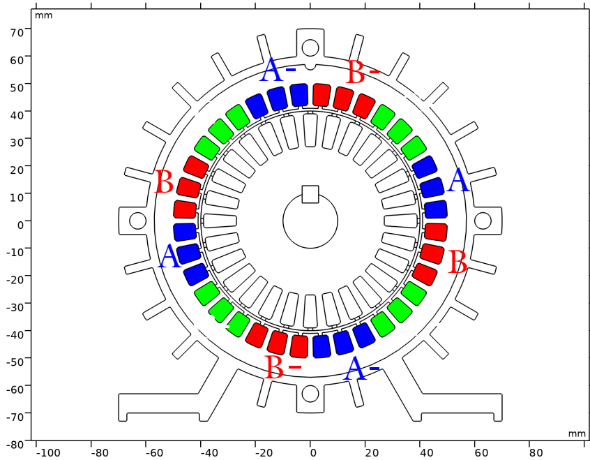
Figure 5: Windings of the 2 pairs pole three-phase induction motor.
