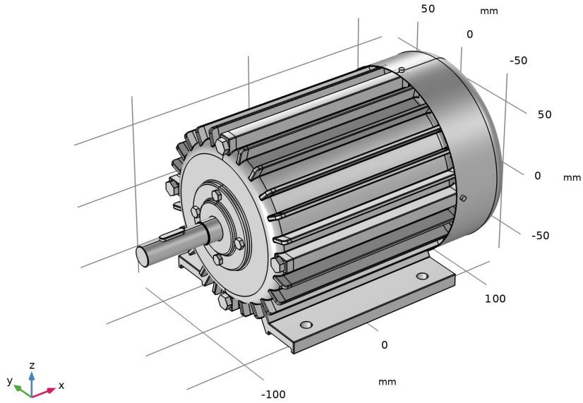
Figure 2: The geometry of a three-phase induction motor housing assembly.
