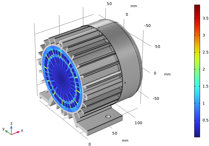
Figure 1: Plot of the magnetic flux density norm on a cross section along the motor displayed at the correct axial position on the 3D geometry.
