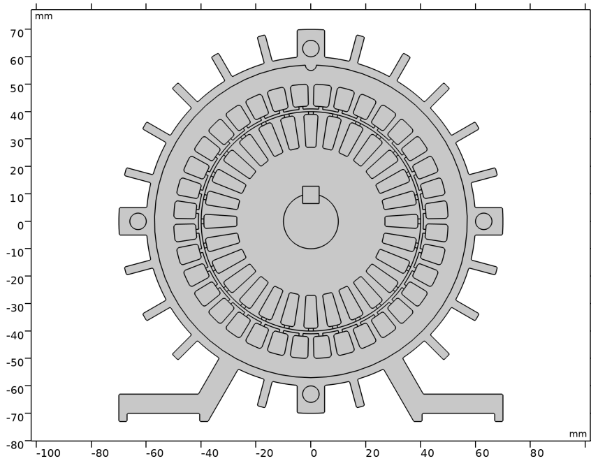
Figure 4: 2D cross section of the induction motor.
