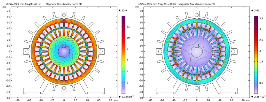
Figure 6: Norm of the magnetic field (surface) and vector potential (contour), z-component, at 0% (left) and 5% slip (right).
