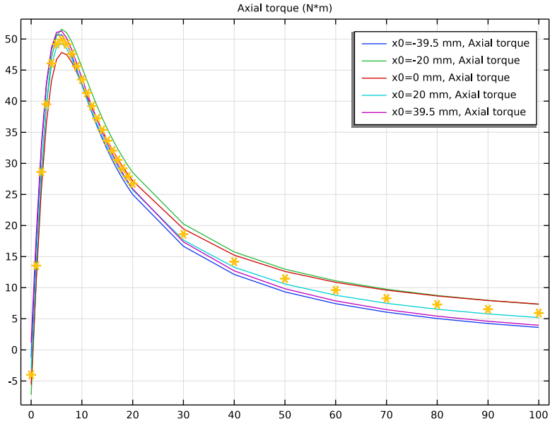
Figure 8: Torque versus slip at five different cut sections within the motor and average value (dashed).
