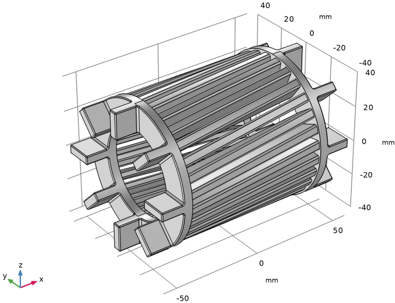
Figure 3: Skewed squirrel cage geometry of the motor.
