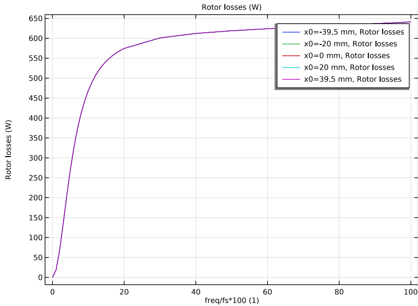
Figure 9: Rotor losses versus slip at five different cut sections within the motor.
