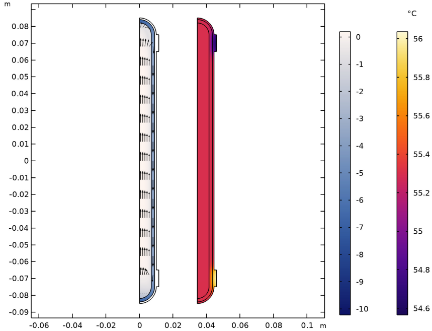
Figure 4: Fluid velocities — \lg(|\mathbf{u}| / \text{m}\cdot\text{s}^{-1}) and temperature in the heat pipe running at the design point.
