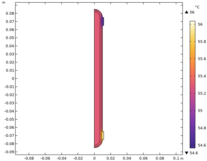
Figure 3: Temperature of heat pipe with saturated wick.
