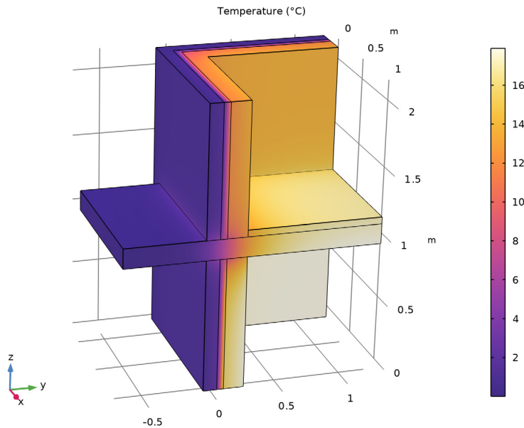
Figure 2: Temperature distribution of ISO 10211:2017 test case 3.
