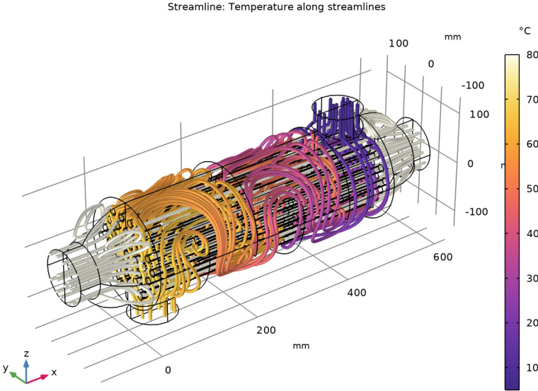
Figure 3: Velocity streamlines.
