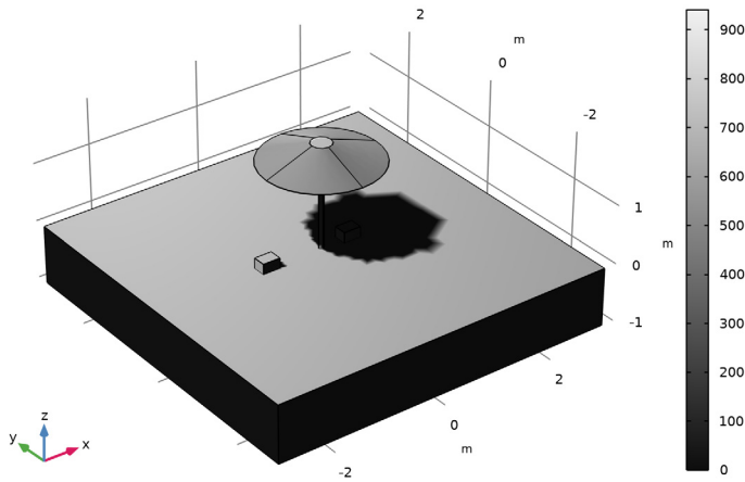
Figure 1: A parasol provides shade on the beach. Two Styrofoam coolers contain beverage cans that should remain as cold as possible.
