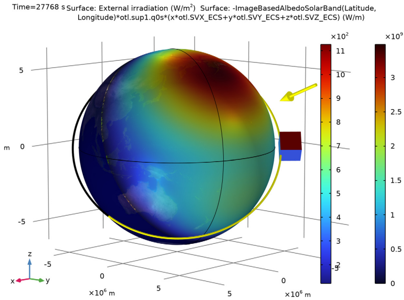
Figure 2: Diffusely reflected solar band flux, the albedo.
